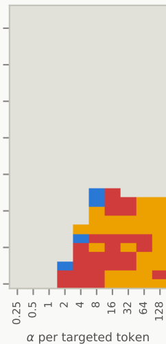
gaussian dropout
