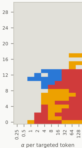
concept direction
