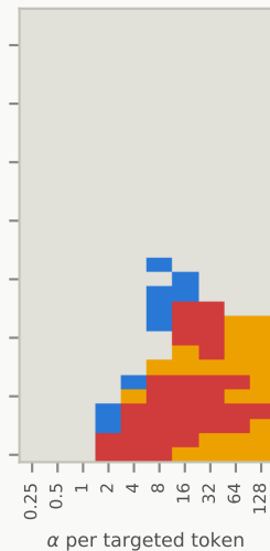
renewed noise
