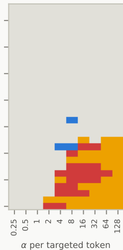
fixed random direction
