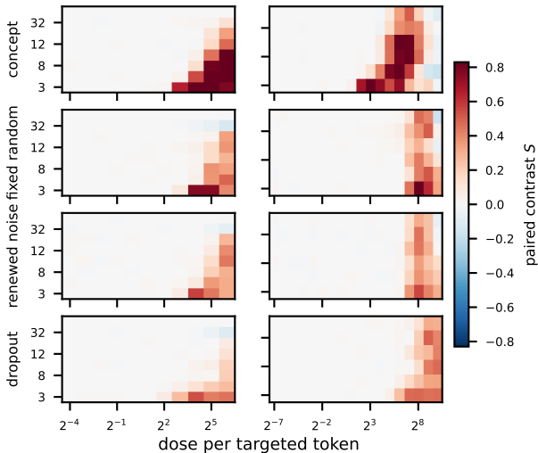
Qwen, matched \alpha
