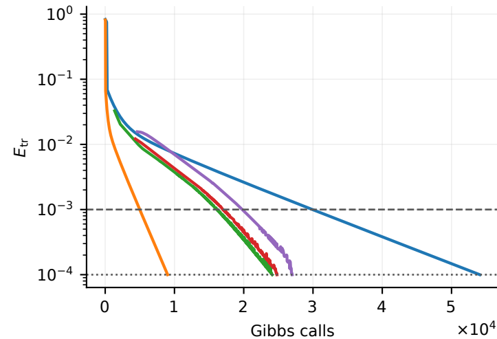
(a) Trace marginal error
