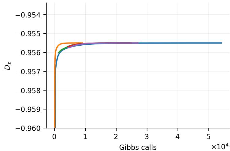
(c) Dual objective
