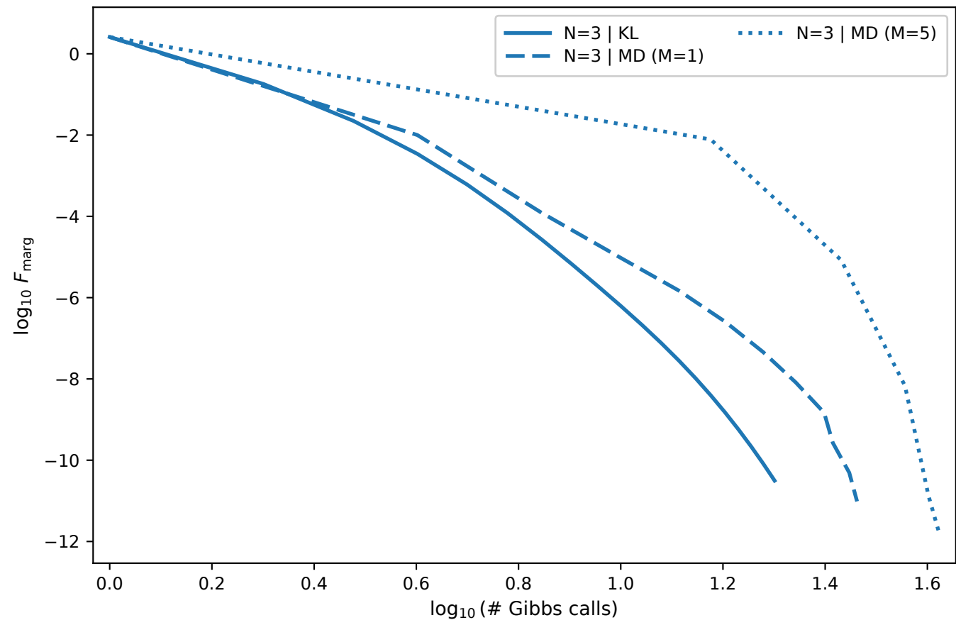
Multi-marginal convergence ( d = 3, \varepsilon = 0.5, N \in \{3\} )
