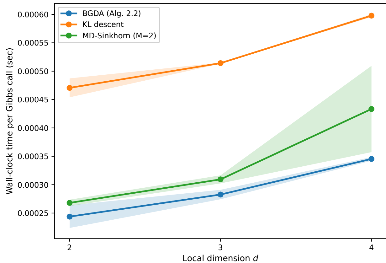
Time per Gibbs call vs d ( N=2 , \varepsilon = 1.0 )
