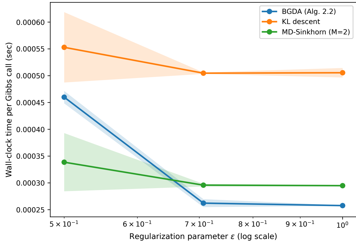
Time per Gibbs call vs \varepsilon ( N=2 , d=3 )
