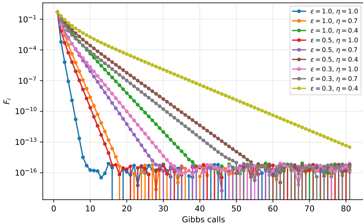
Inner update convergence: F_i vs Gibbs calls
