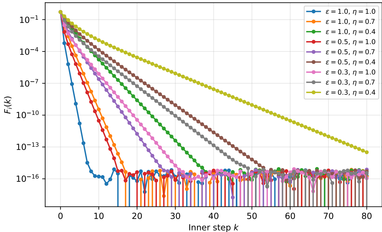
Inner update convergence: F_i = \text{KL}(\rho_i \parallel \gamma_i) vs step
