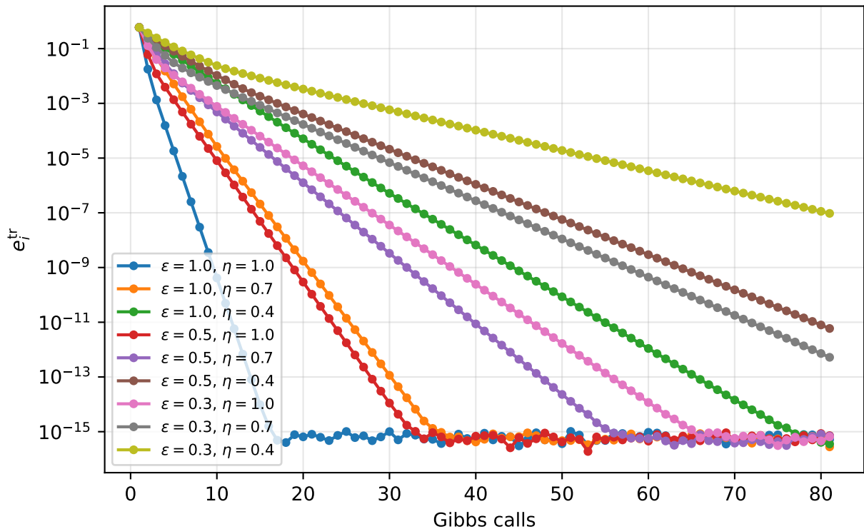
Inner update convergence: e_i^{\text{tr}} vs Gibbs calls
