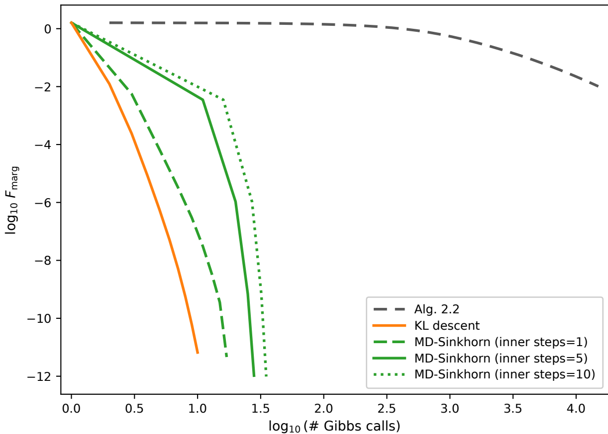
Convergence for entropic QOT ( d = 5 , \varepsilon = 0.5 )
