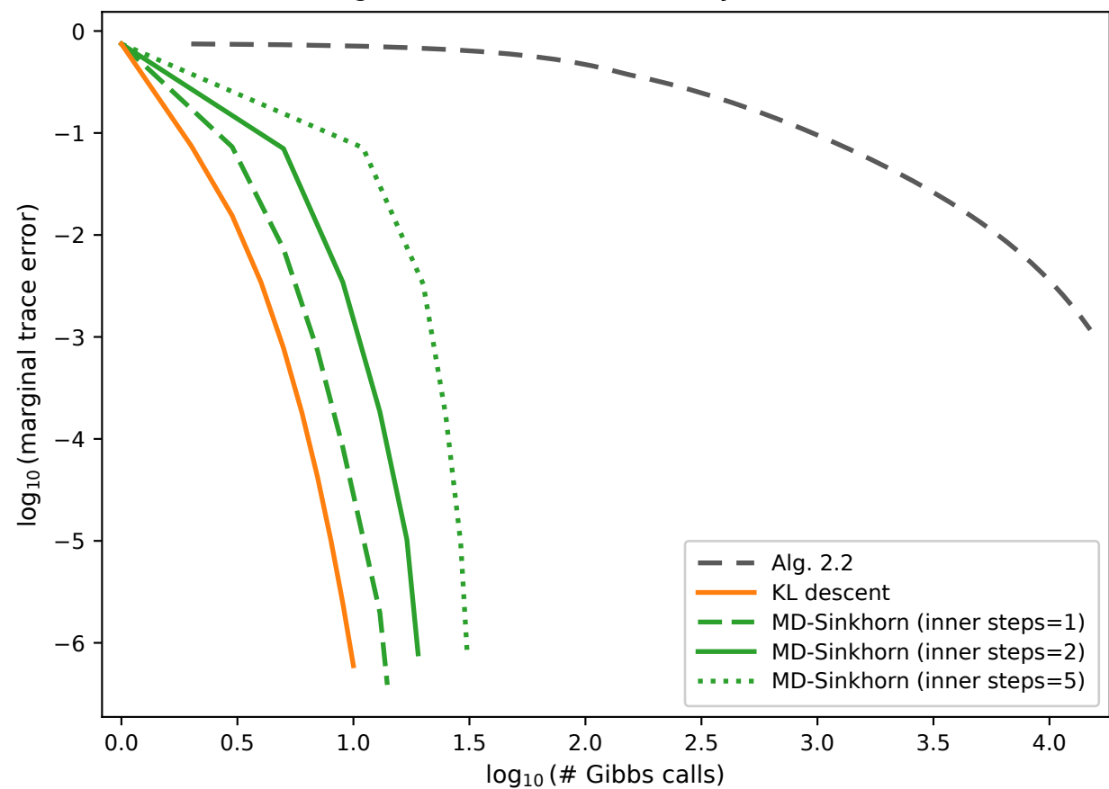
Convergence (trace-norm feasibility) ( d = 3 , \varepsilon = 0.5 )
