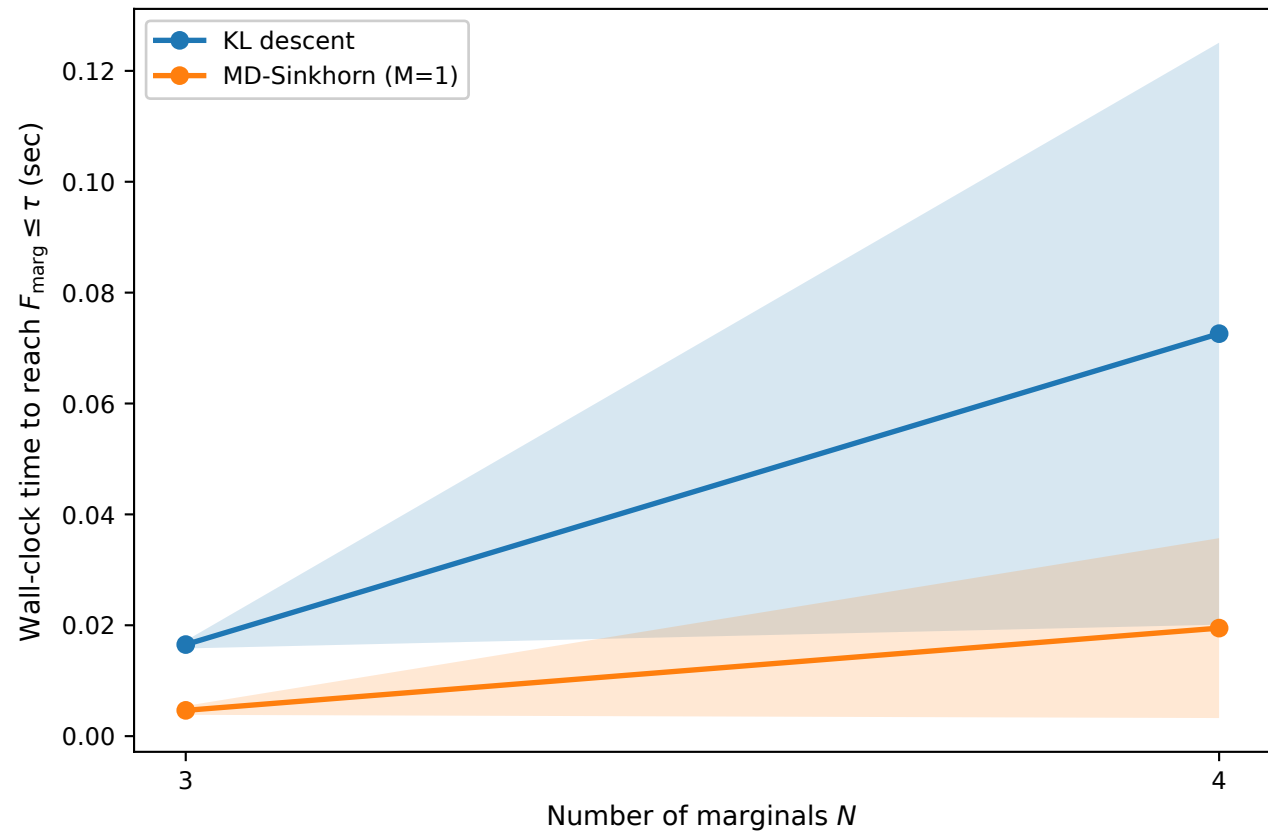
Multi-marginal scaling ( d = 2, \varepsilon = 1.0, \tau = 10^{-8} )
