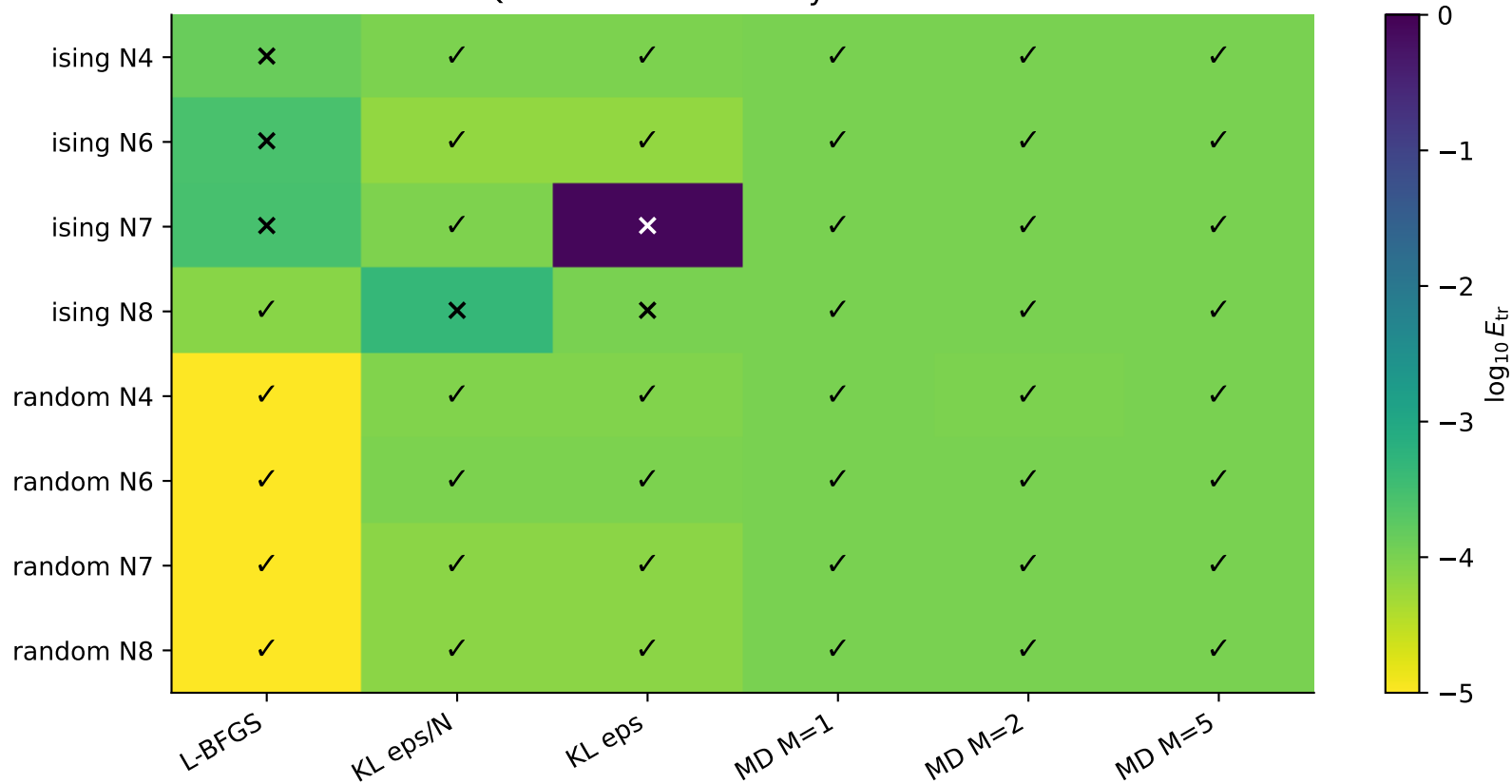
Qubit mixed feasibility at \varepsilon = 10^{-3}
