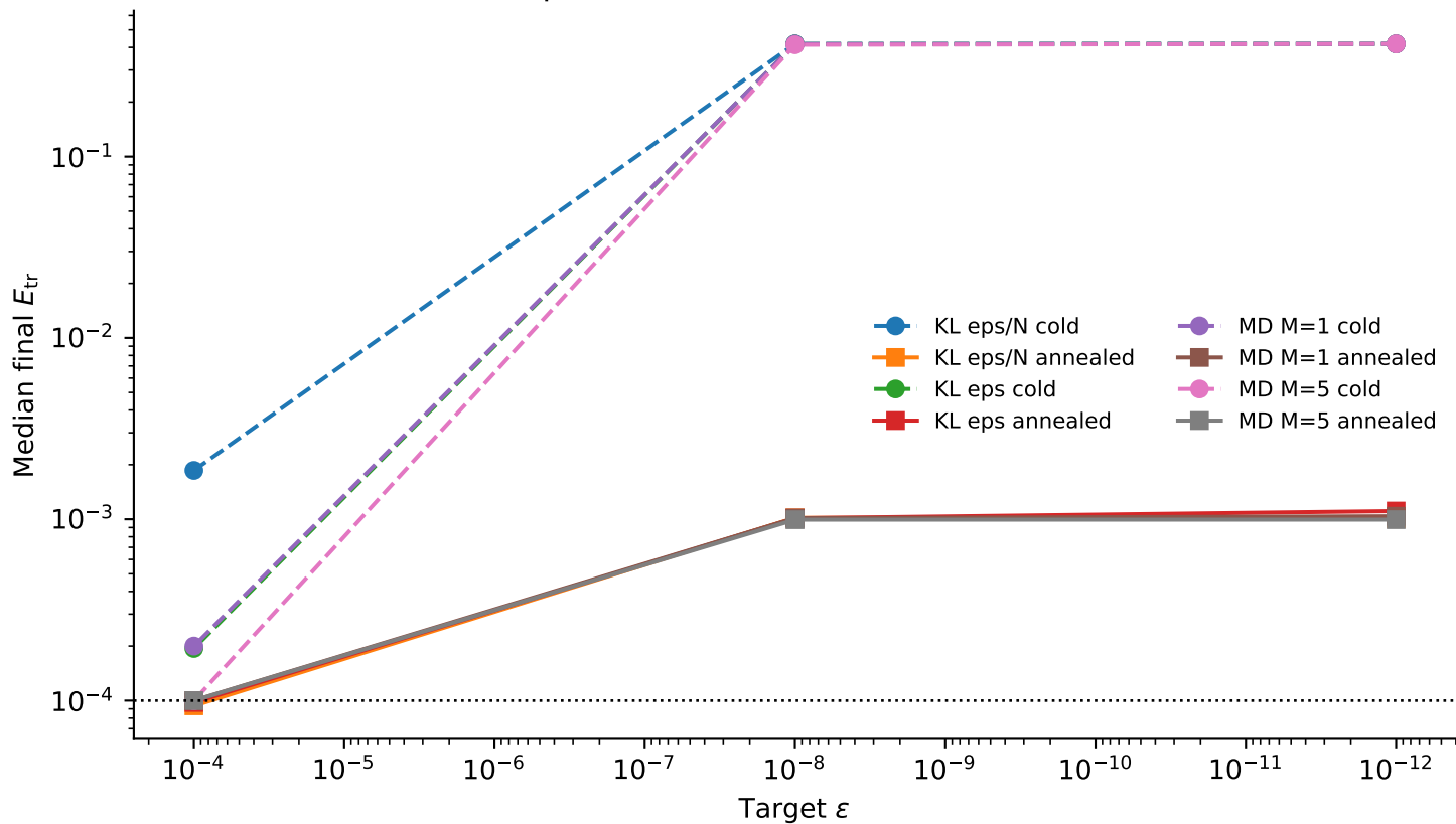
Small-epsilon final error: cold versus annealed
