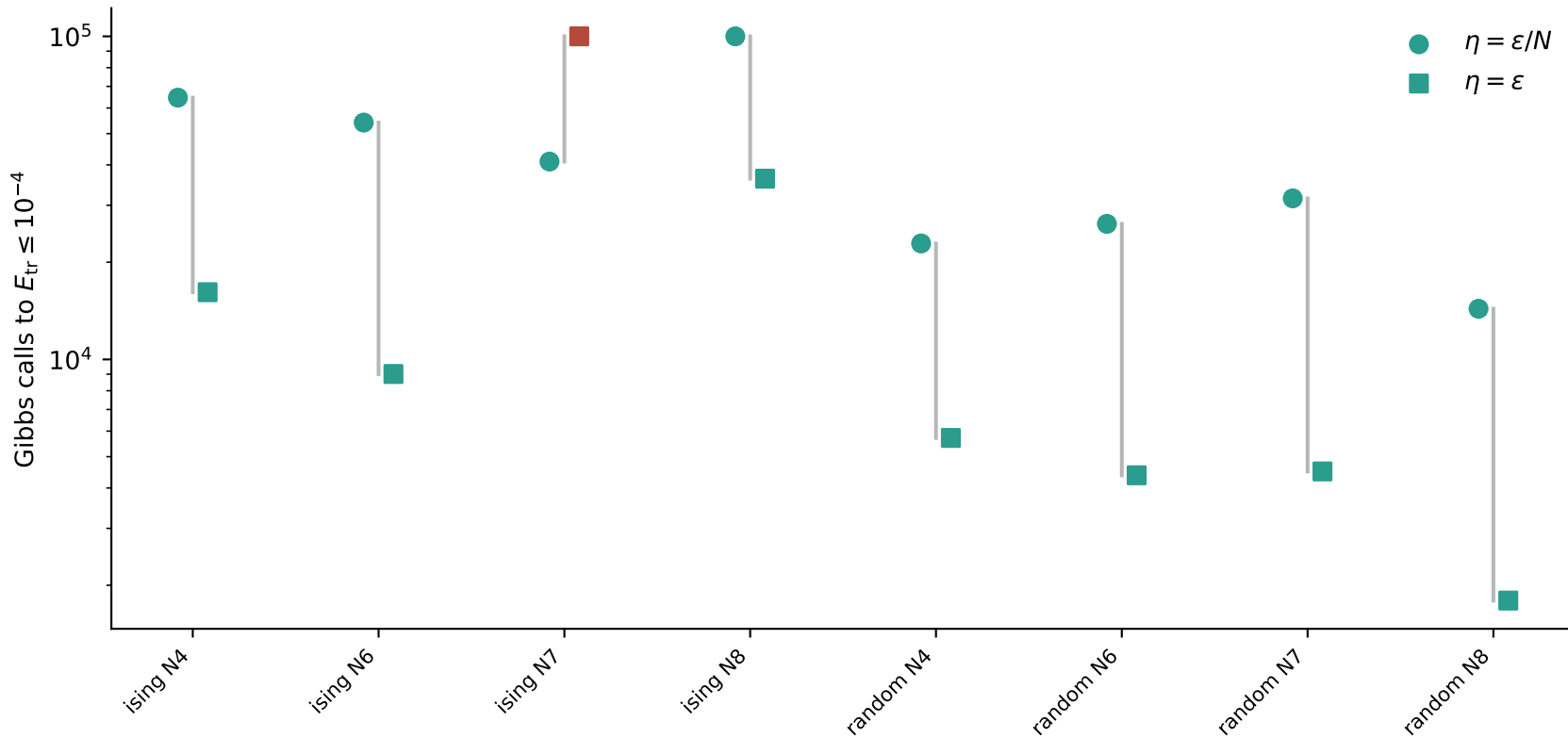
KL step-size comparison on qubit mixed benchmarks, \varepsilon = 10^{-3}
