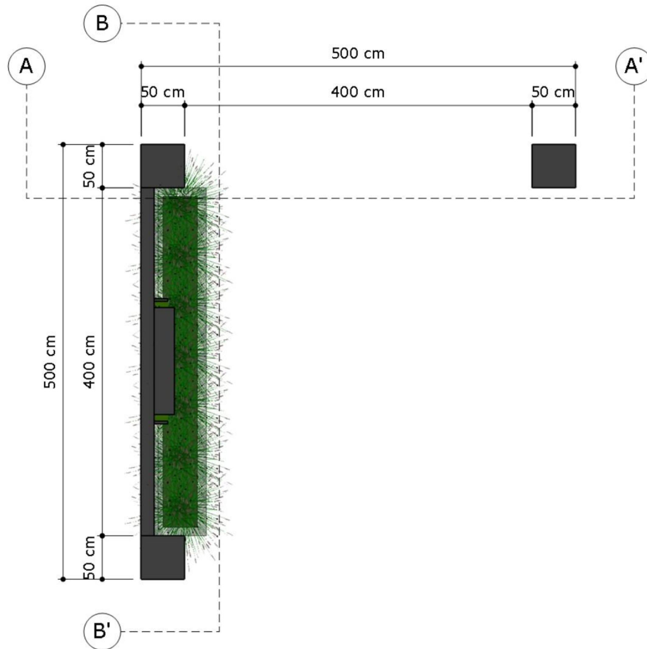
FLOOR PLAN 1 : 30 SCALE
