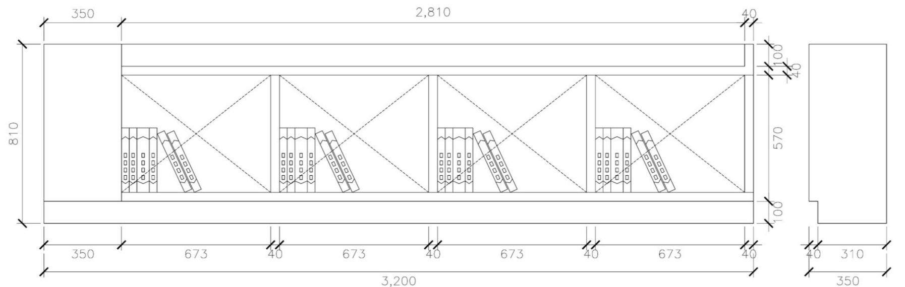
TAMPAK A (TYPE 2) SCALE 1:10
