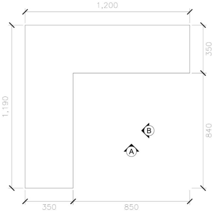
LEMARI BUKU (TYPE 1) SCALE 1:10
