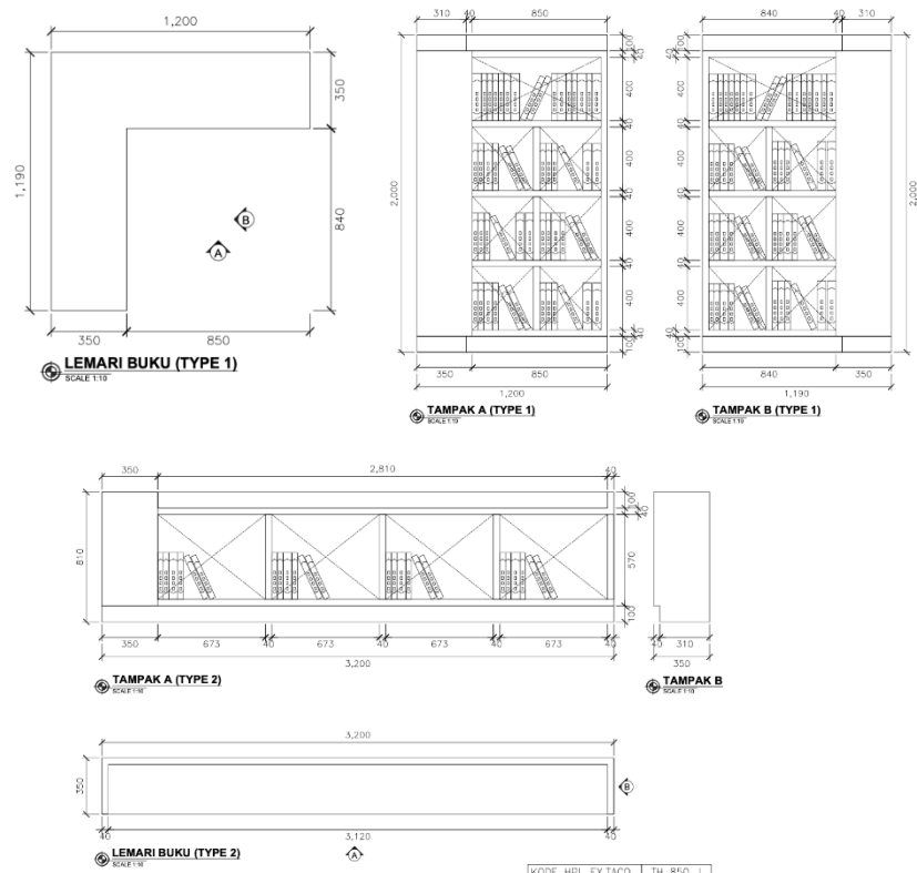
Gambar 3.8. Gambar Detail Lemari
