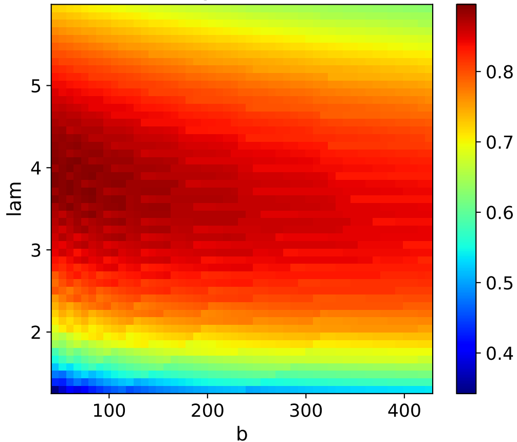
Original model
