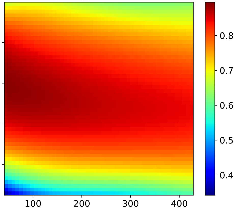
gPC approximation
