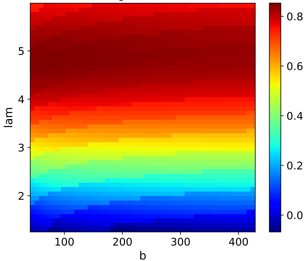
Original model
