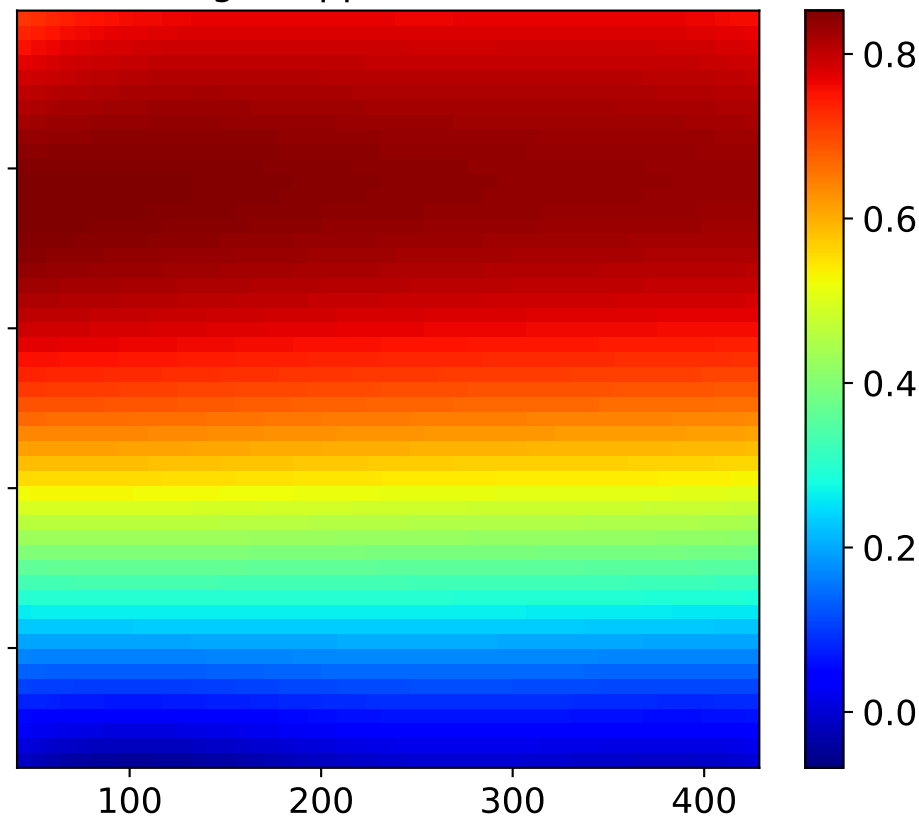
gPC approximation
