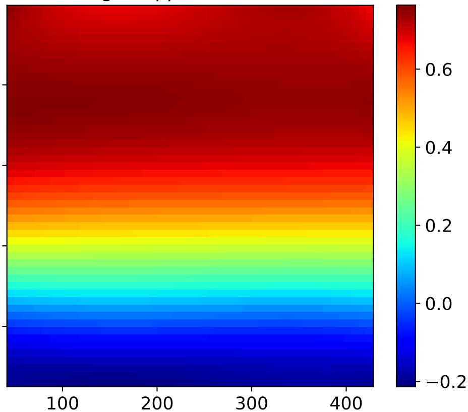
gPC approximation
