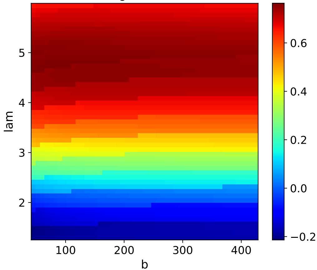
Original model
