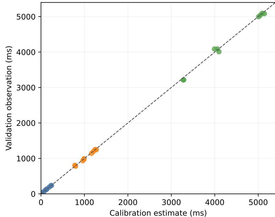
Expected TTFT
