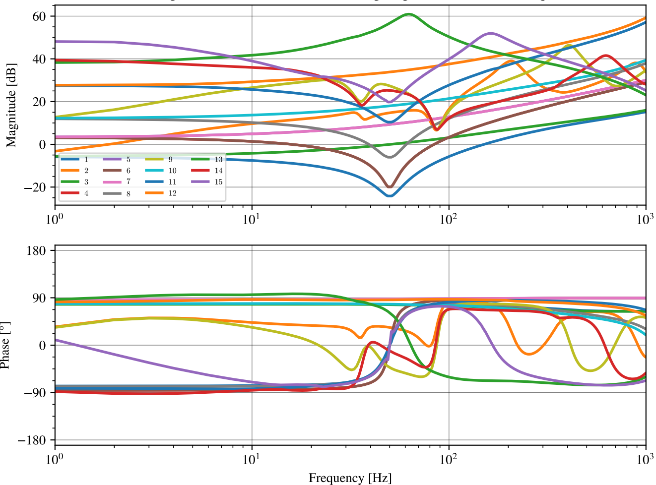
Modal impedance: EVD of the closed-loop impedance over 576 frequencies
