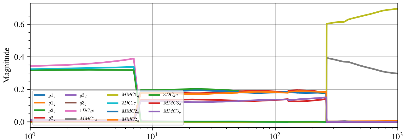
Sensitivity of the largest closed-loop modal impedance w.r.t. its diagonal elements
