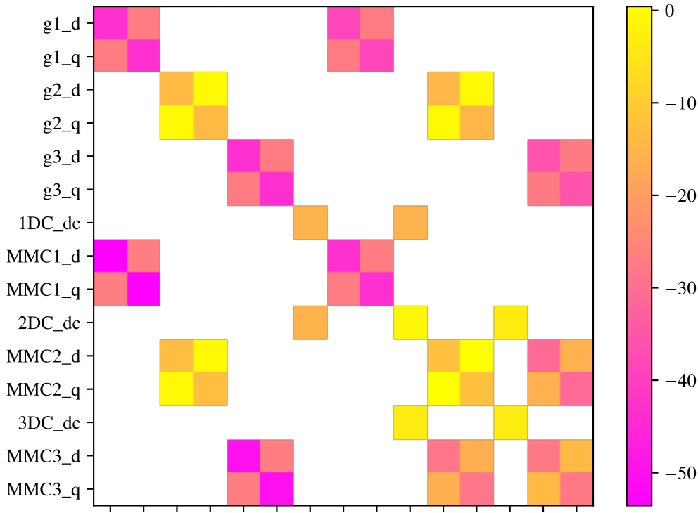
Edge admittance matrix at 1.0 Hz
