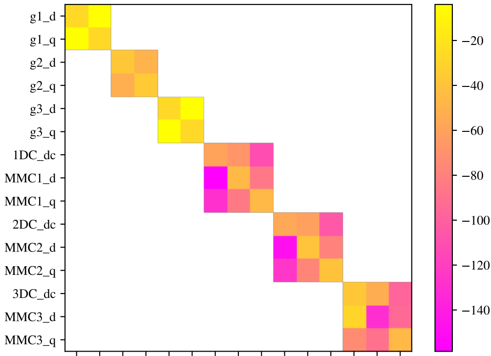
Node admittance matrix at 1.0 Hz
