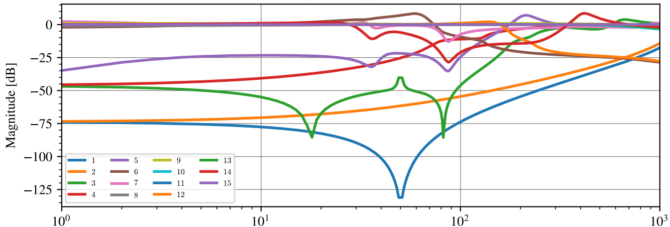
Bode plot of 1/(1 + \lambda(L)) over 576 frequencies
