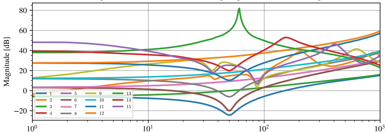
Modal impedance: EVD of the closed-loop impedance over 576 frequencies
