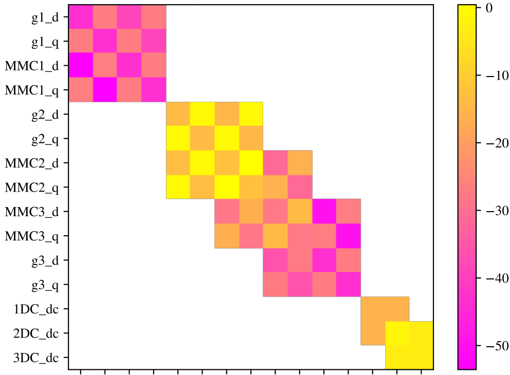
Auxiliary edge admittance matrix at 1.0 Hz
