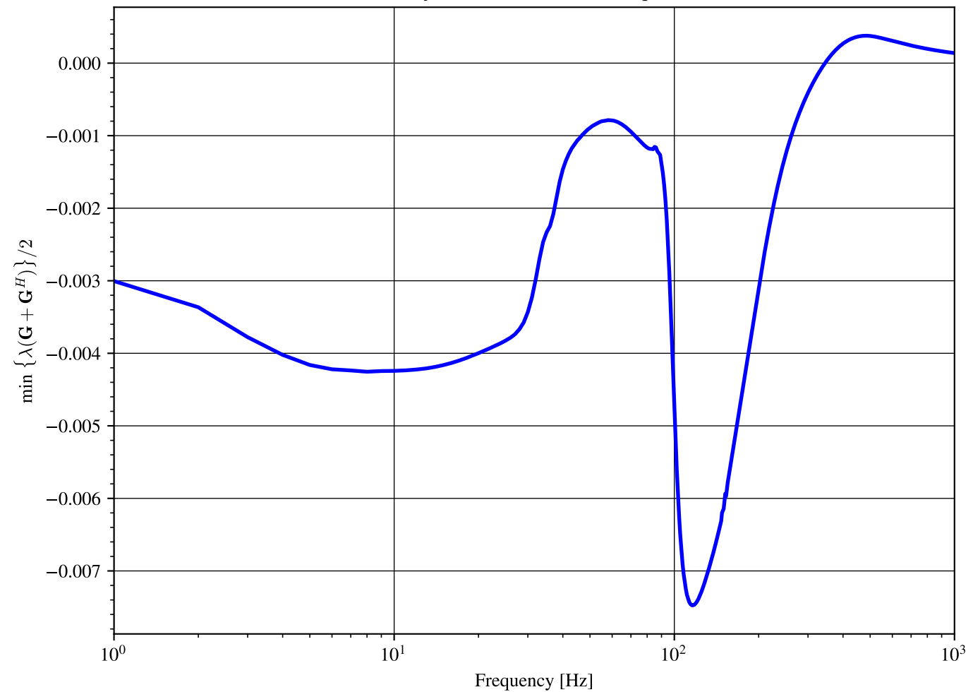
Passivity evaluation for 576 frequencies
