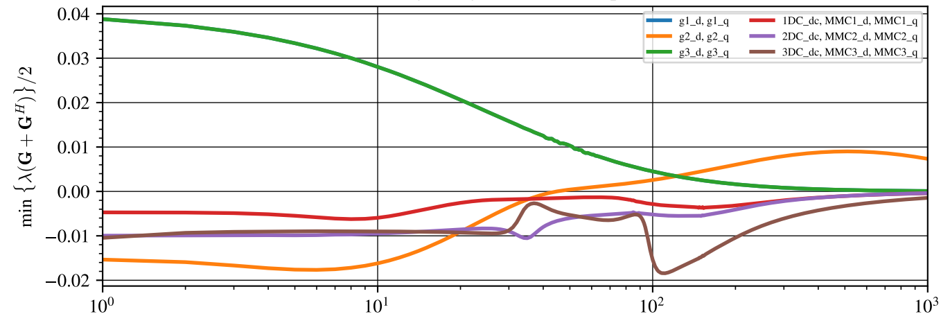
Passivity analysis for 576 frequencies
