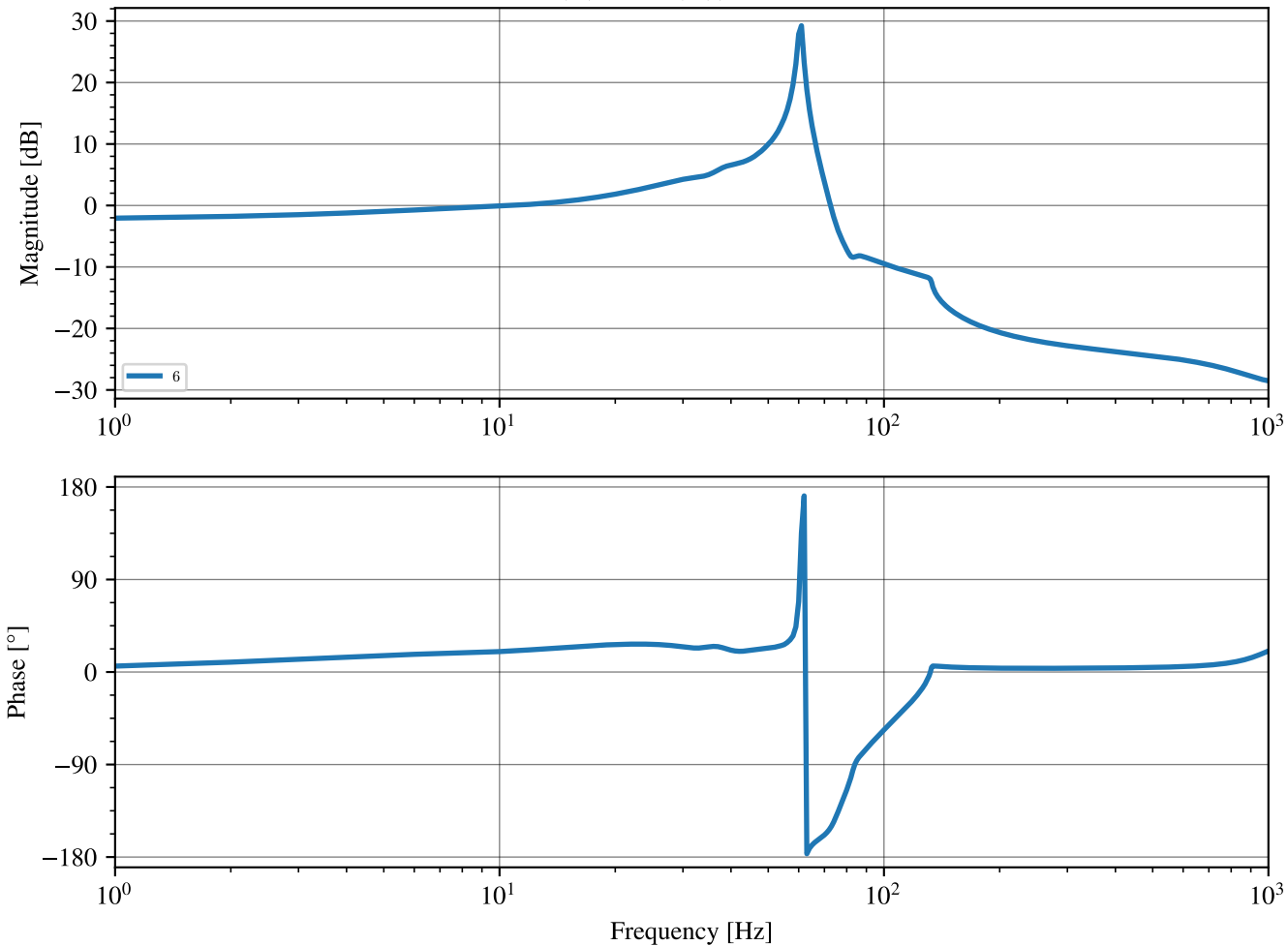
Bode plot of 1/(1 + \lambda_6(L)) over 576 frequencies
