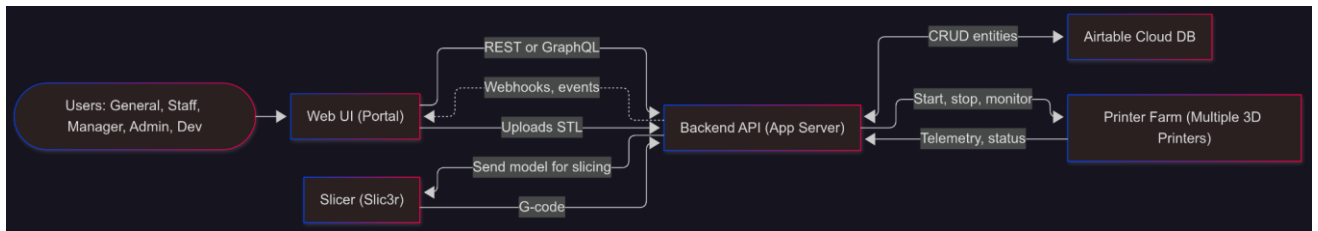
Figure 2. D1 – Major Subsystems and Data Flow.
