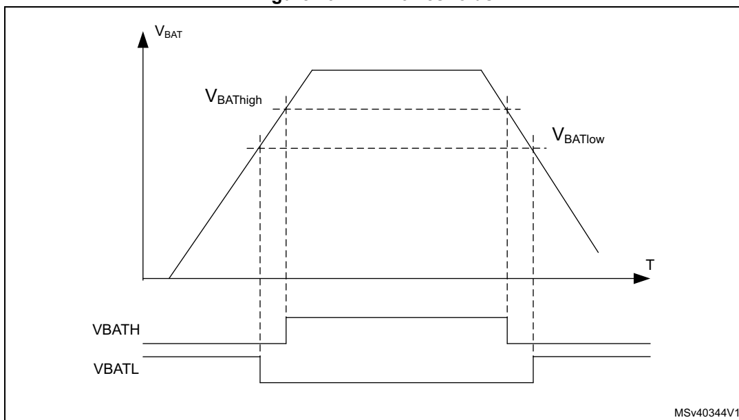
Figure 29. VBAT thresholds
