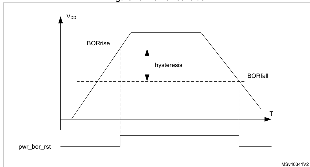
Figure 26. BOR thresholds
