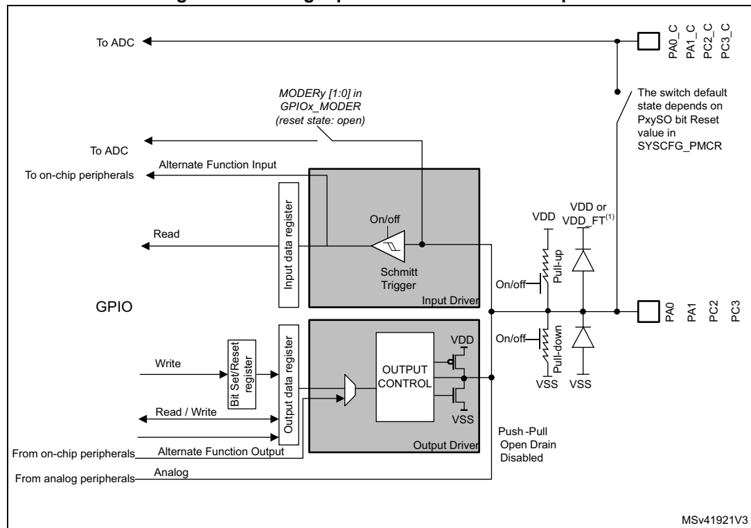
Figure 77. Analog inputs connected to ADC inputs
