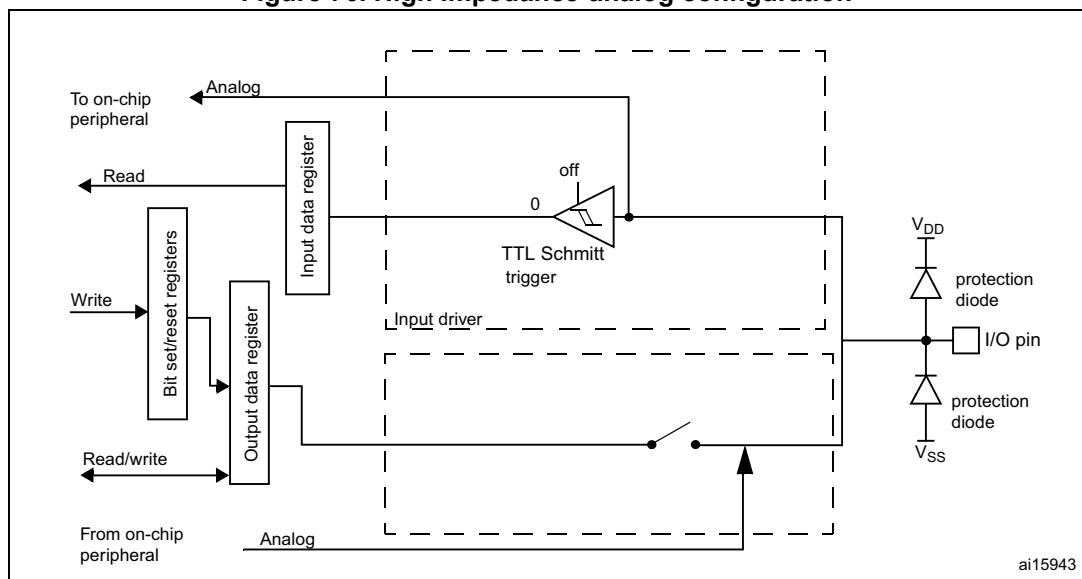
Figure 76. High impedance-analog configuration
