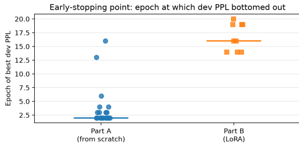
Figure 2: Epoch at which dev PPL bottomed out (early-stopping point). The from-scratch models overfit within \sim 2 epochs; the LoRA adapters keep improving for far longer.
