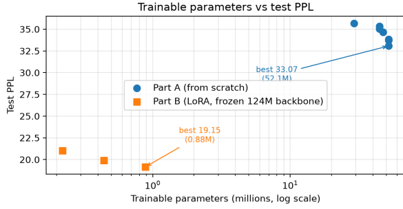
Figure 1: Trainable parameters vs test PPL. Part B (LoRA) reaches far lower PPL with two orders of magnitude fewer trainable parameters, on top of a frozen 124M pre-trained backbone.
