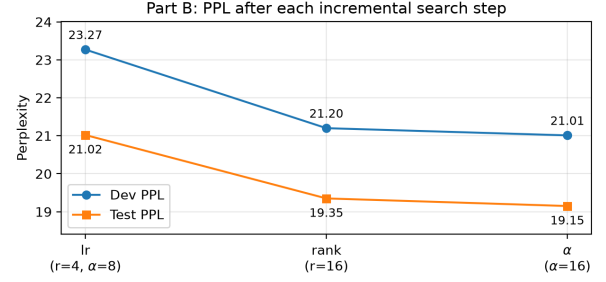
Figure 2: Part B: dev and test PPL after each incremental search step (learning rate, rank, then \alpha ).
