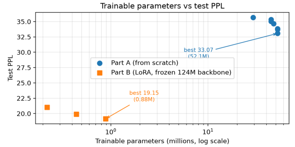
Figure 3: Trainable parameters vs test PPL. Part B (LoRA) reaches far lower PPL with two orders of magnitude fewer trainable parameters, on top of a frozen 124M pre-trained backbone.
