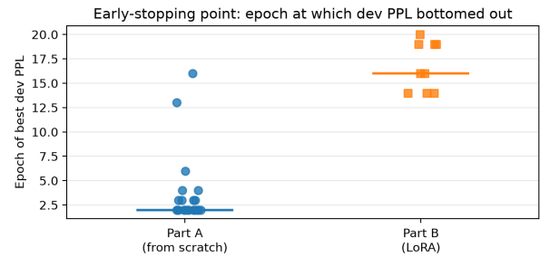
Figure 4: Epoch at which dev PPL bottomed out (early-stopping point). The from-scratch models overfit within \sim 2 epochs; the LoRA adapters keep improving for far longer.
