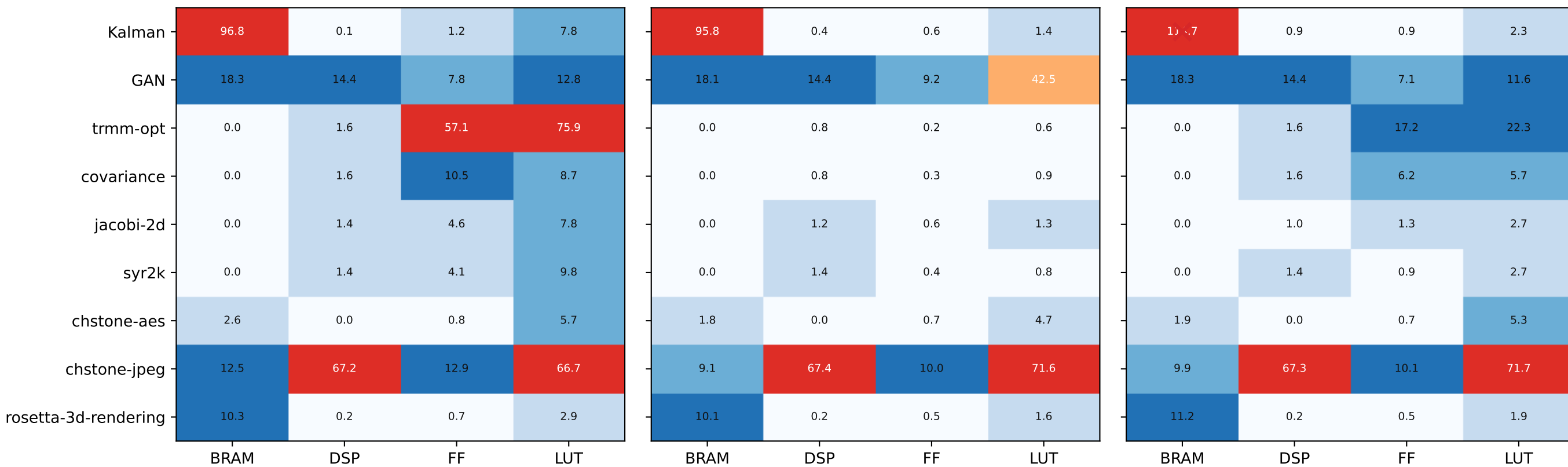
LATENCY
