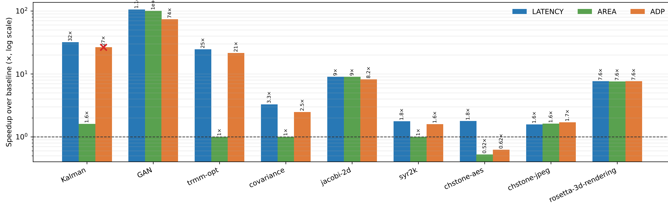
LATENCY
