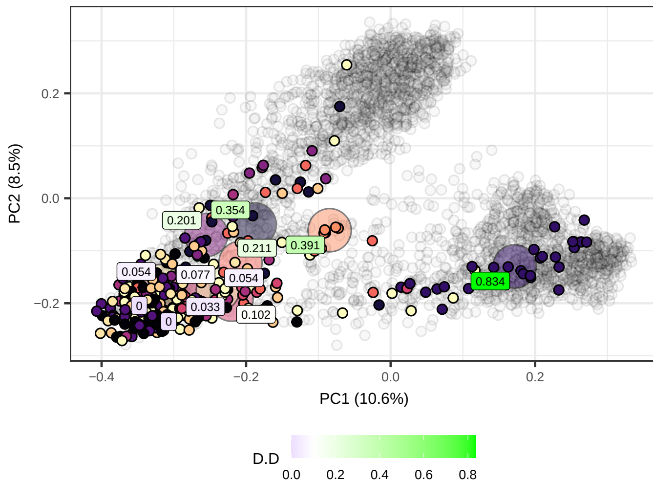
Unweighted UniFrac PCoA with 11 Pre-FMT Clusters Centers and Dysbiosis Scores
