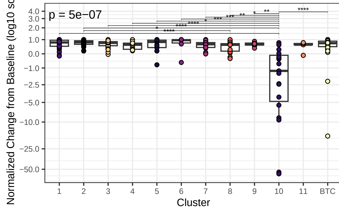
Normalized Delta Dysbiosis Scores of 11 Clusters Matched Pre- & Post-FMT
