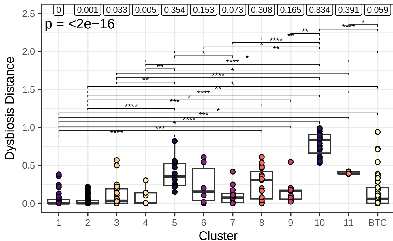
Matched FMT Baseline Dysbiosis Distances of 11 Clusters 237 Patients
