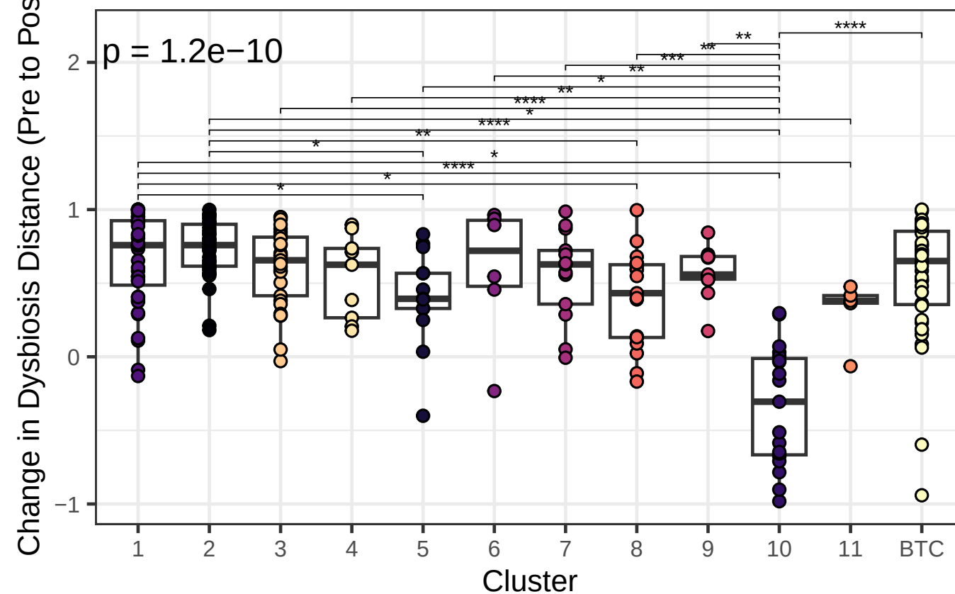
Change in Dysbiosis Distances of 11 Clusters Matched Pre- & Post-FMT
