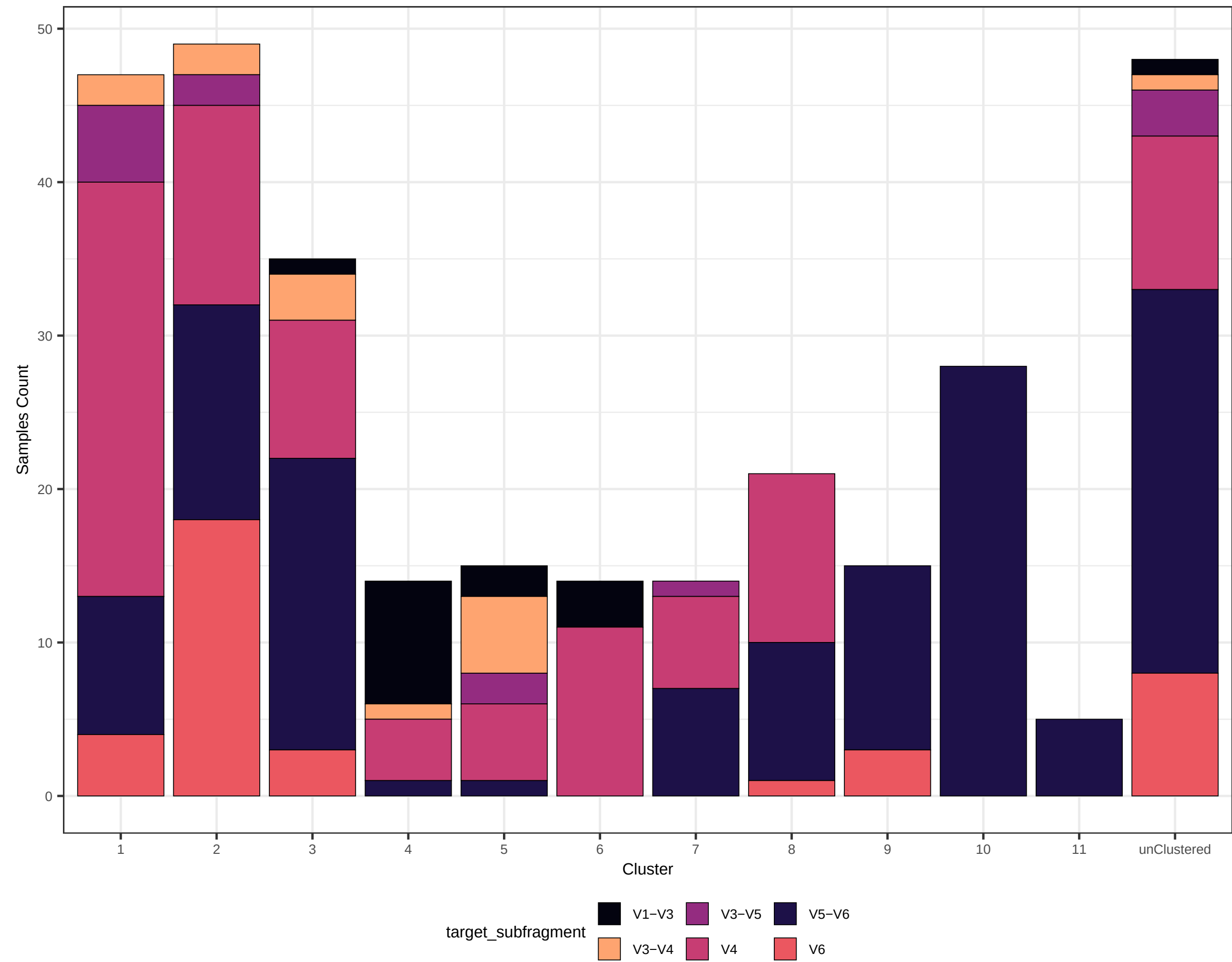
Samples from Each of 11 Dysbio Clusters By Subfragment
