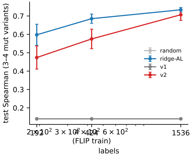
GB1 four-site landscape (FLIP two-vs-rest)
