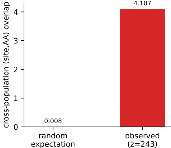
parallel evolution (8 populations)
