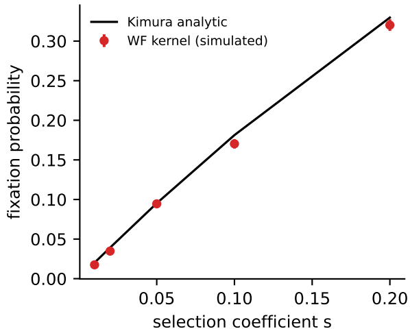
fixation probability vs Kimura
