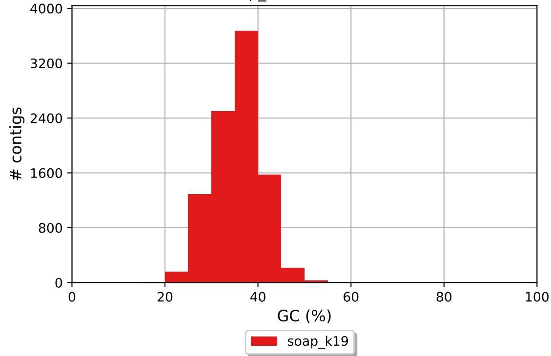
soap_k19 GC content
