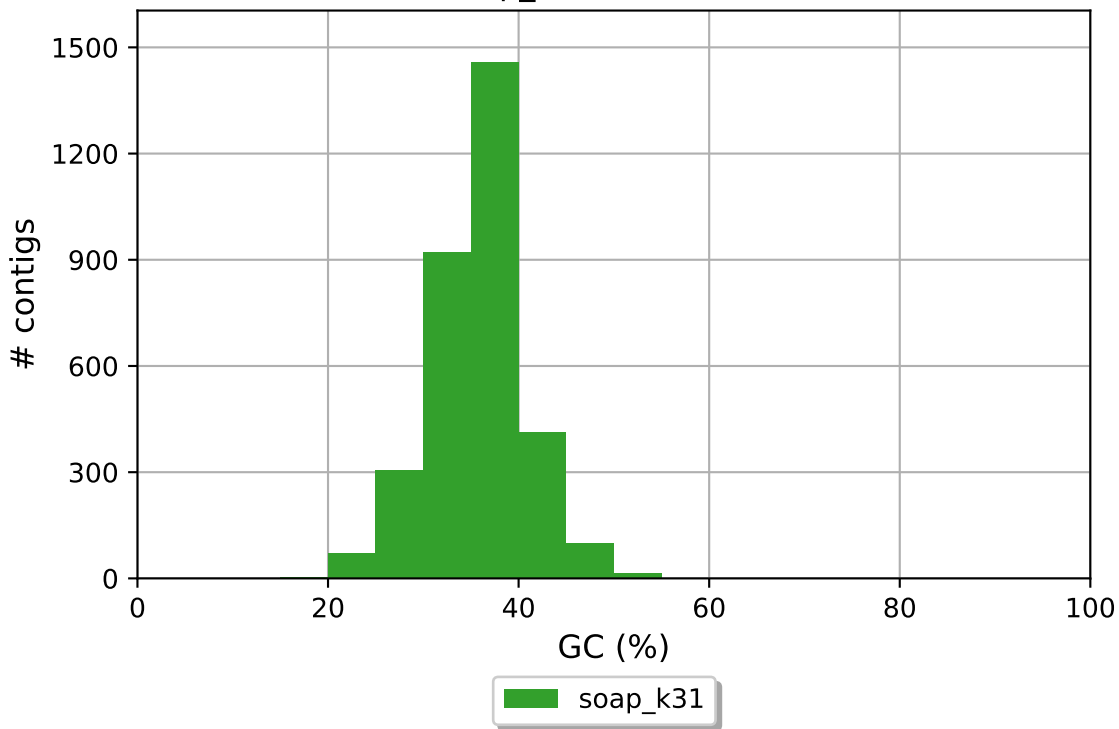
soap_k31 GC content
