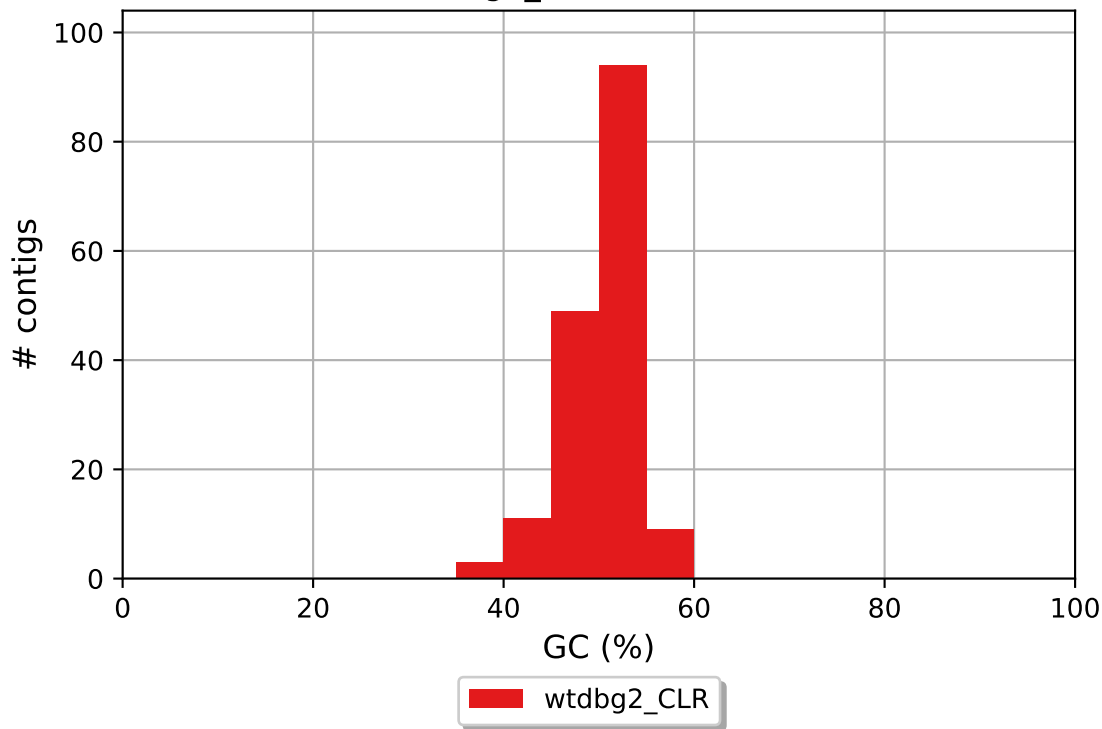
wtdbg2_CLR GC content
