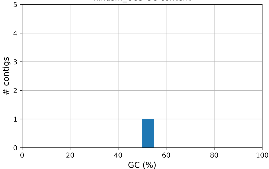
hifiasm_CCS GC content
