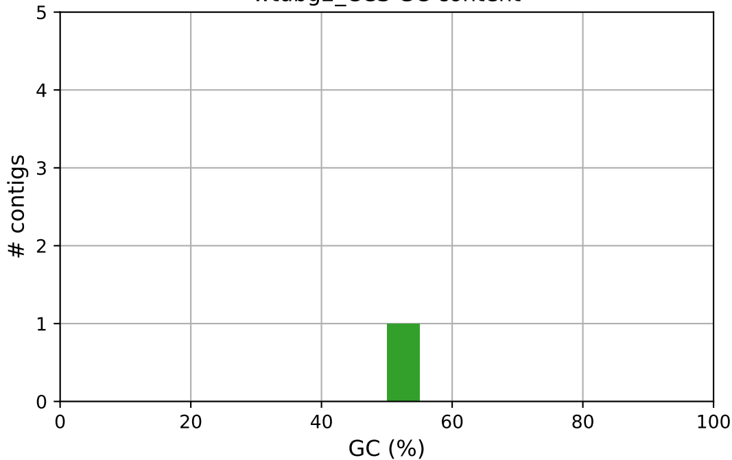
wtdbg2_CCS GC content
