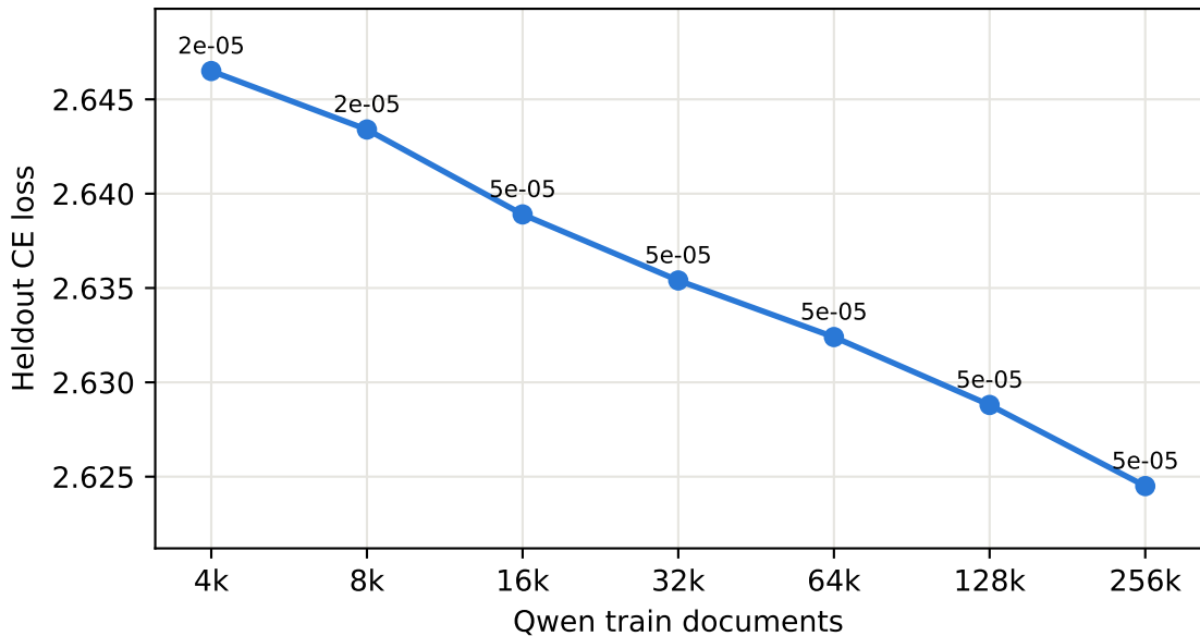
Qwen2.5-1.5B selected LR heldout trend
