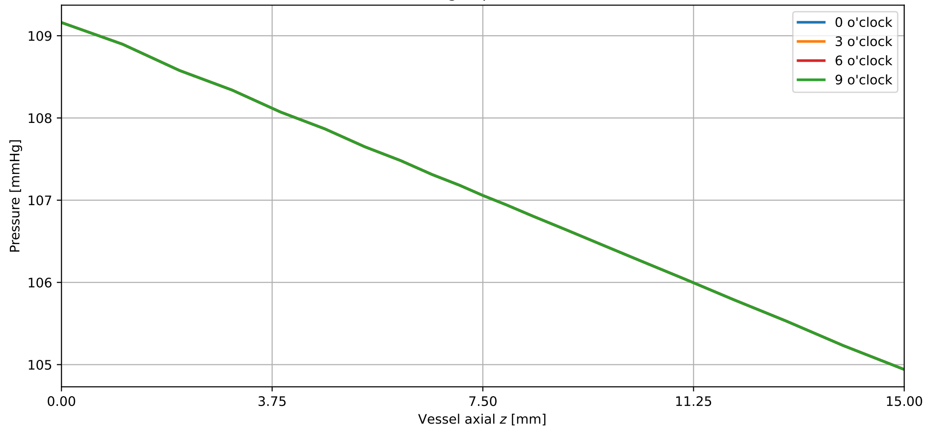
Time-averaged pressure at wall
