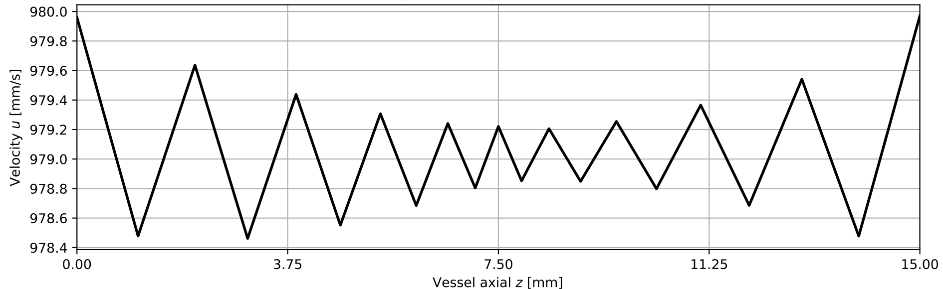
Time-averaged velocity at location: 0, center, :
