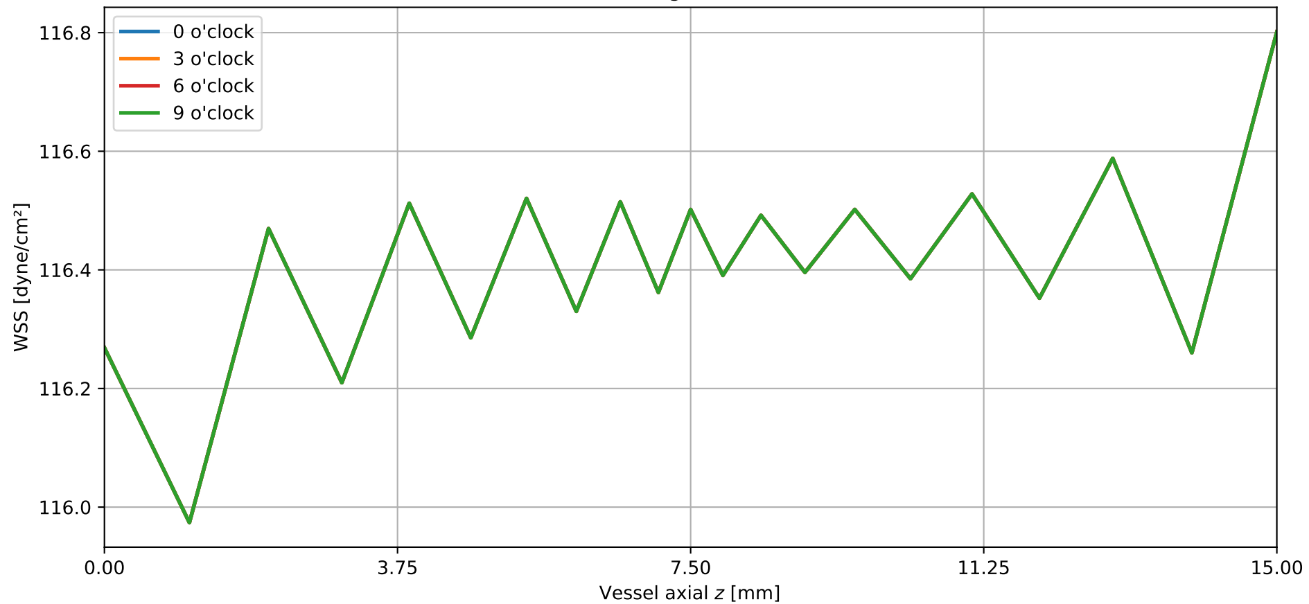
Time-averaged wss at wall
