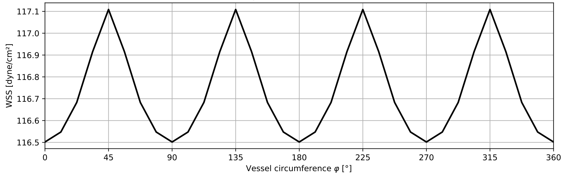
Time-averaged wss at location: :, wall, mid
