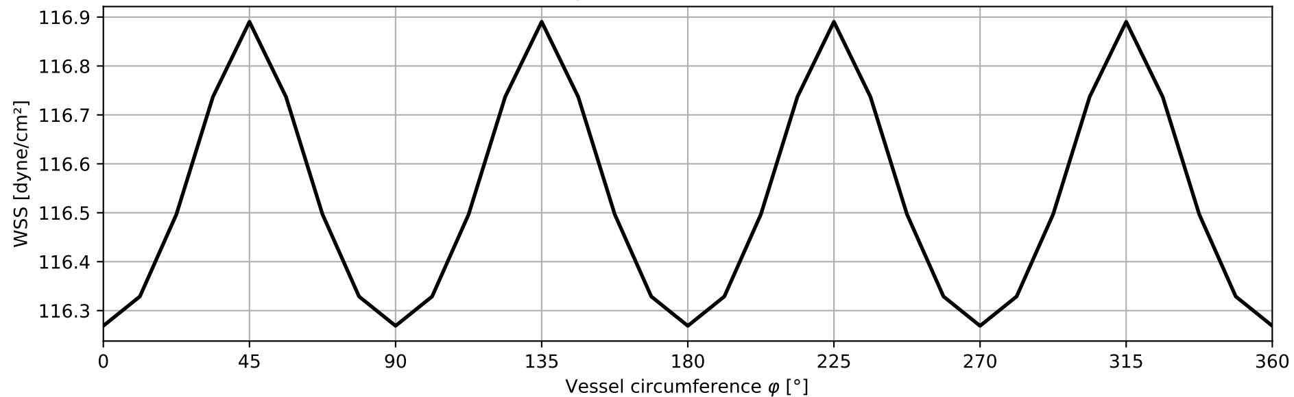
Time-averaged wss at location: :, wall, start
