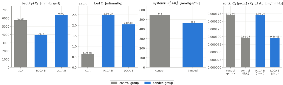
Settled calibration knobs ( R_p+R_d and C ; band S excluded): control vs banded
