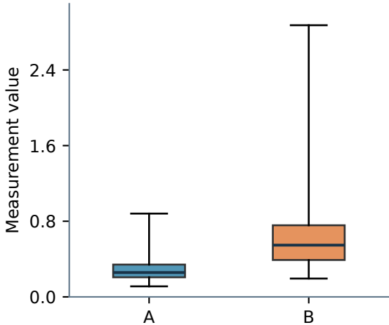
c Box plot
