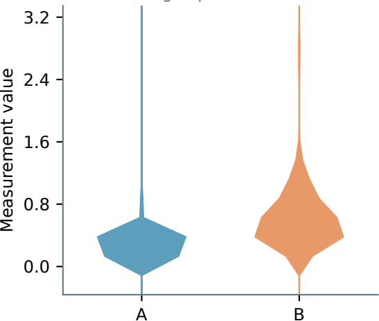
f Violin plot
