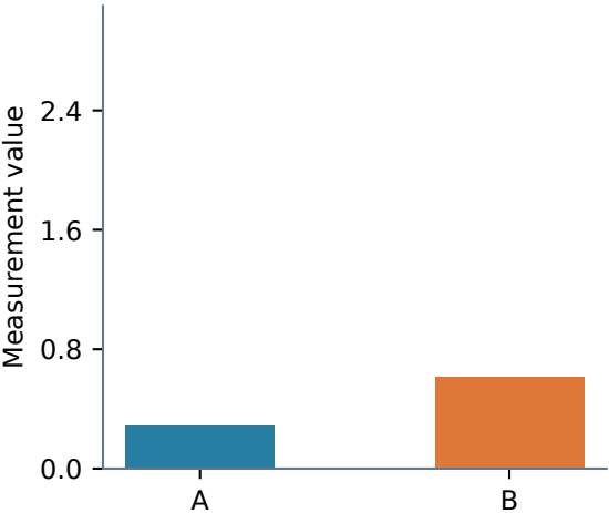
a Bar chart
