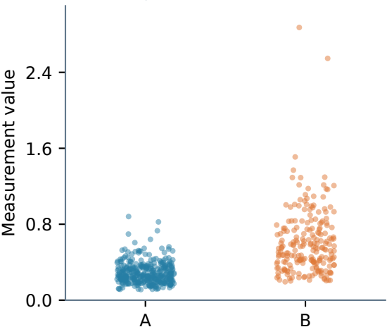
e Dot plot
