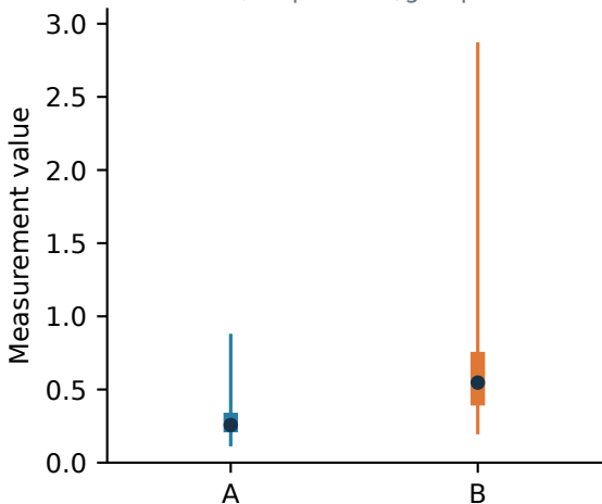
g Error-bar / interval plot
