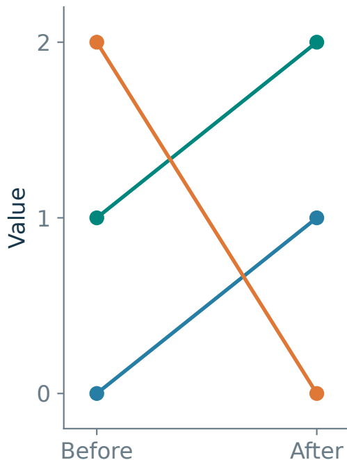
b Permuted pairs
