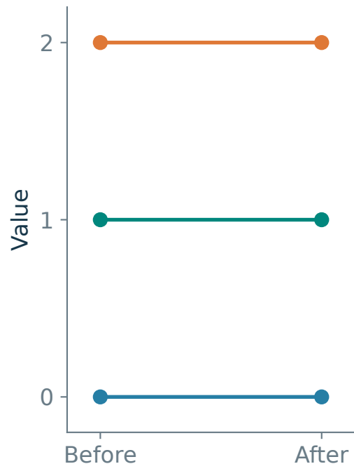
a Aligned pairs
