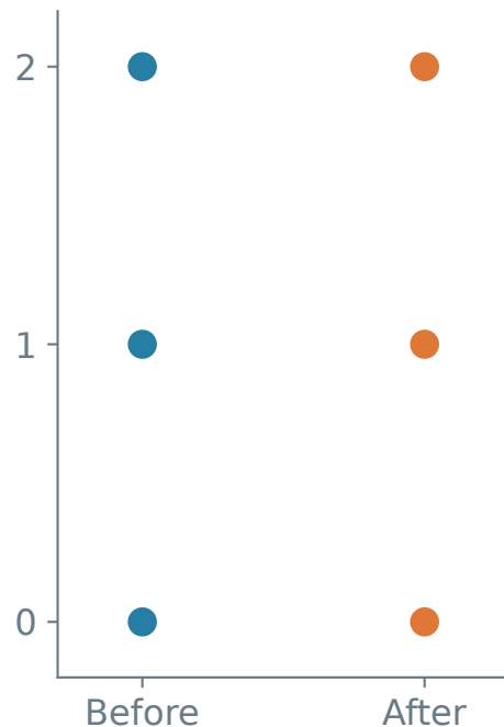
c Identical marginals
